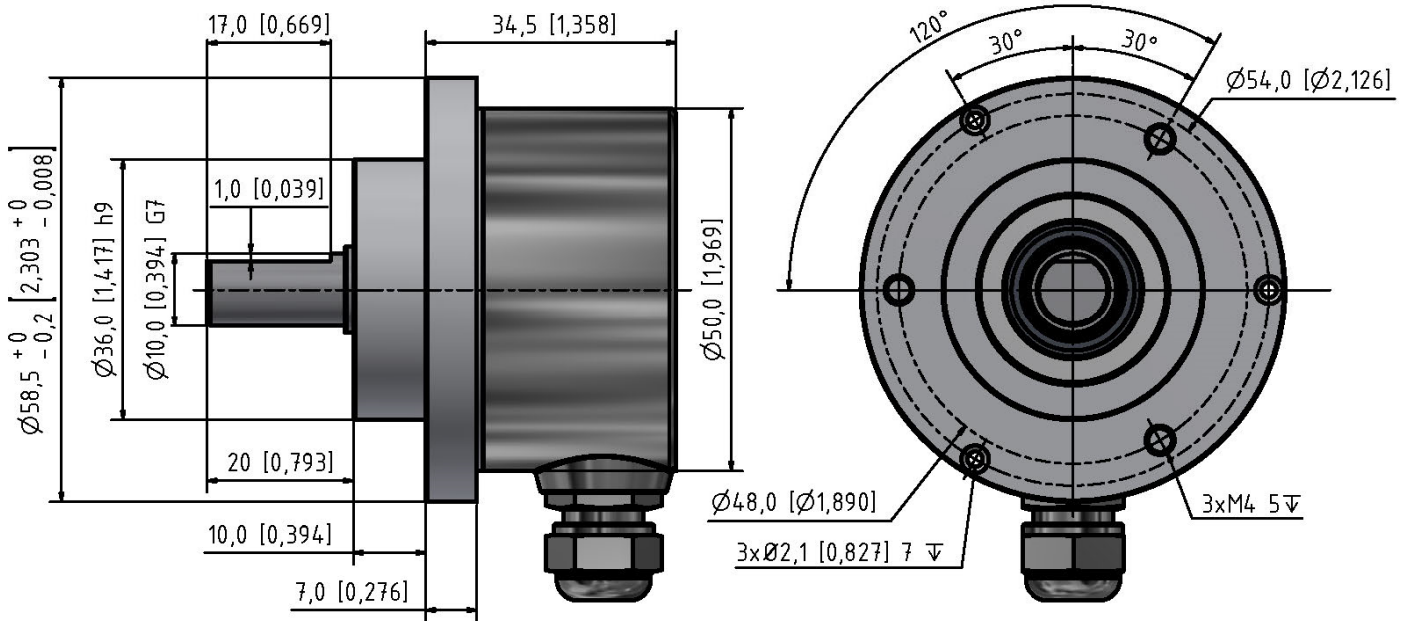
Standard Cable Gland (axial or radial outlet) mm [inches]
