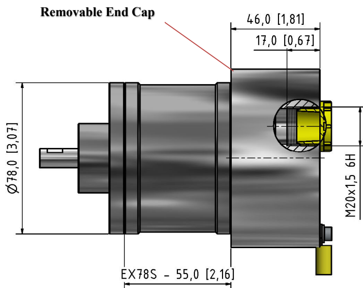
Back Round End Cap (FG)
