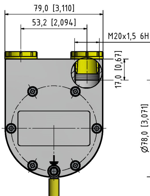
Side Standard End Cap (FZ)
