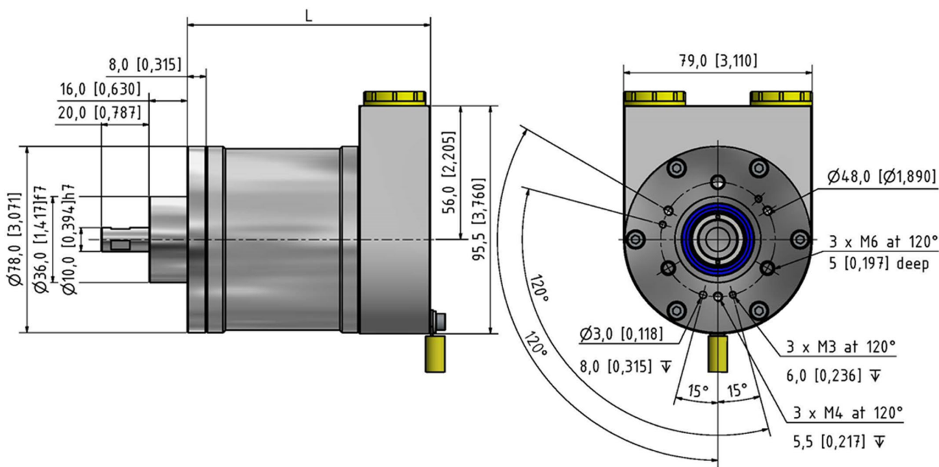
Face Mount C Clamping Flange
