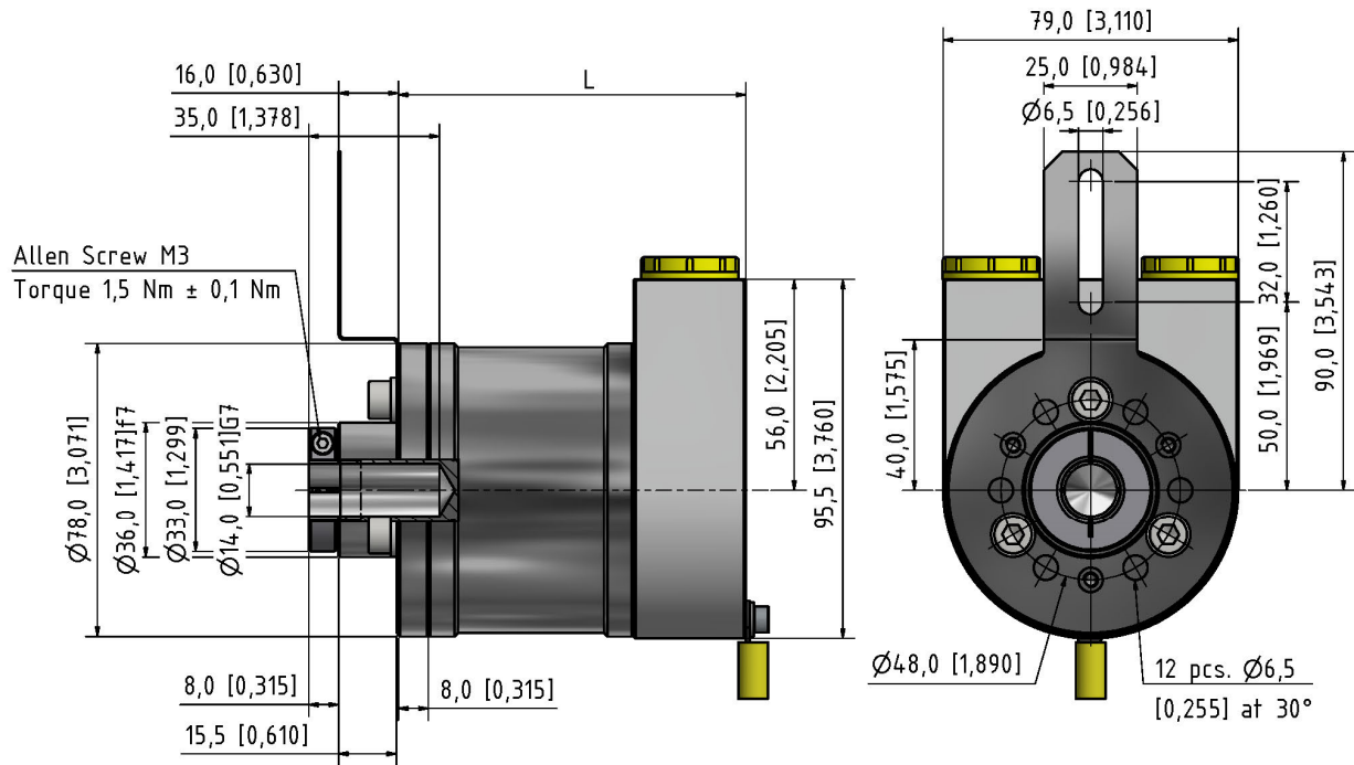
Face Mount C Clamping Flange
