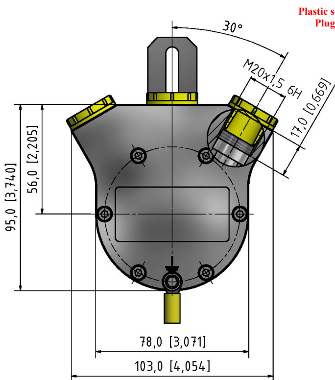
Side Triple End Cap (FE)
