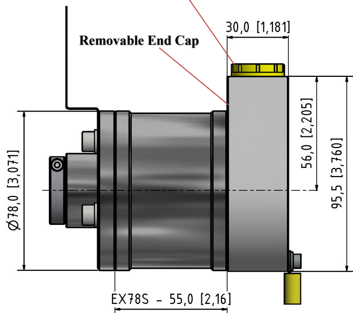
Side Standard End Cap (FZ)
